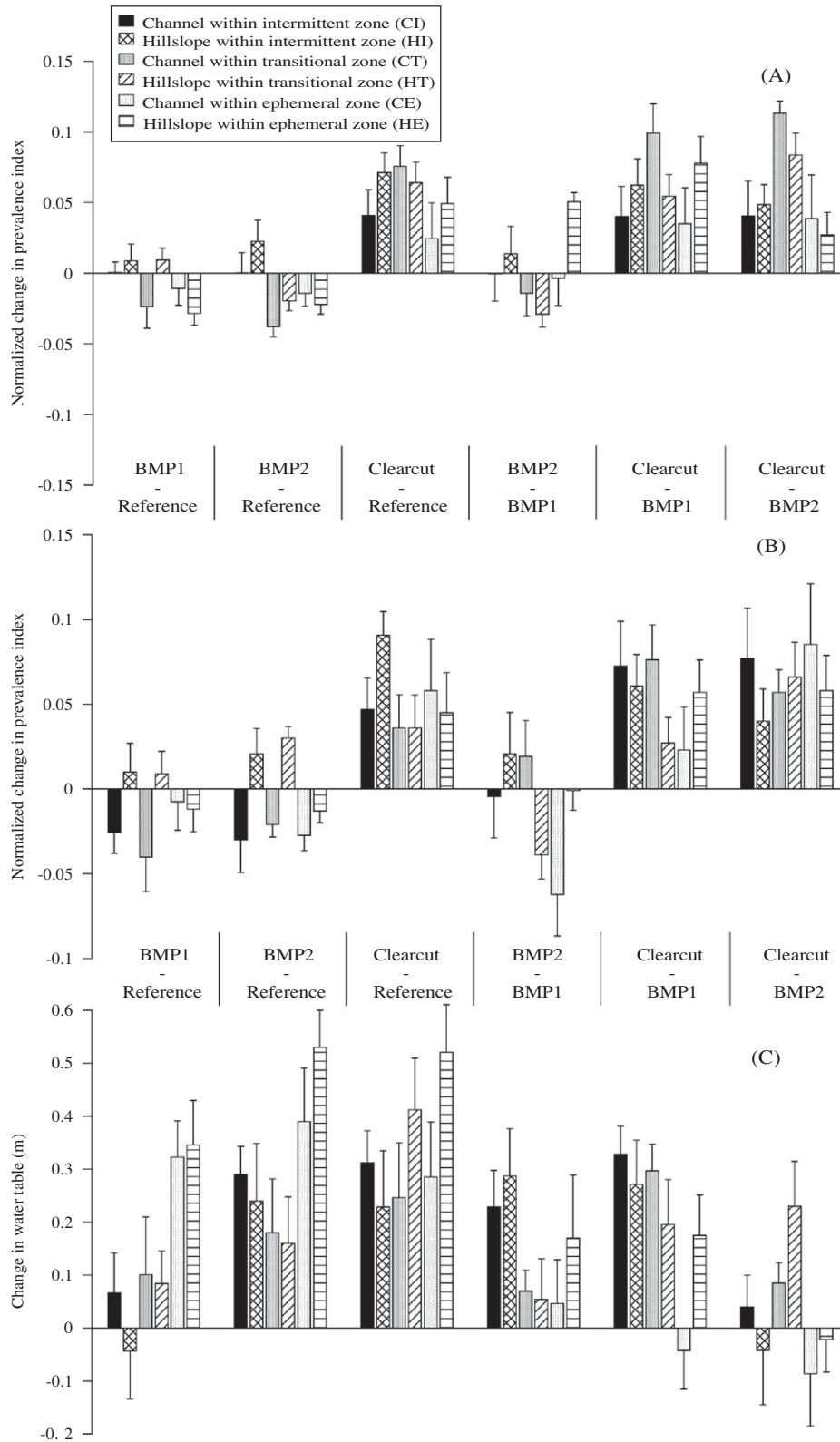
Fig. 4. Pairwise comparisons by treatment for change in mean water table and mean PI in small headwater streams of Webster County, Mississippi. Graph (A) comparisons between prevalence index (PI) of plots across all strata at the same topographic positions. Graph (B): comparisons between prevalence index (PI) of plots for understory stratum at the same topographic positions. Graph C: comparisons of change in water table (DWT) among plots at the same topographic positions. Pairwise comparison was conducted between the two listed treatments (i.e. top minus bottom). For pairwise comparisons of normalized change in PI, positive PI values indicate a shift toward drier species assemblages and negative values indicate a shift toward wetter species assemblages. For pairwise comparisons of change in water table, positive values indicate a shift toward higher water table and negative values indicate a shift toward lower water table.
