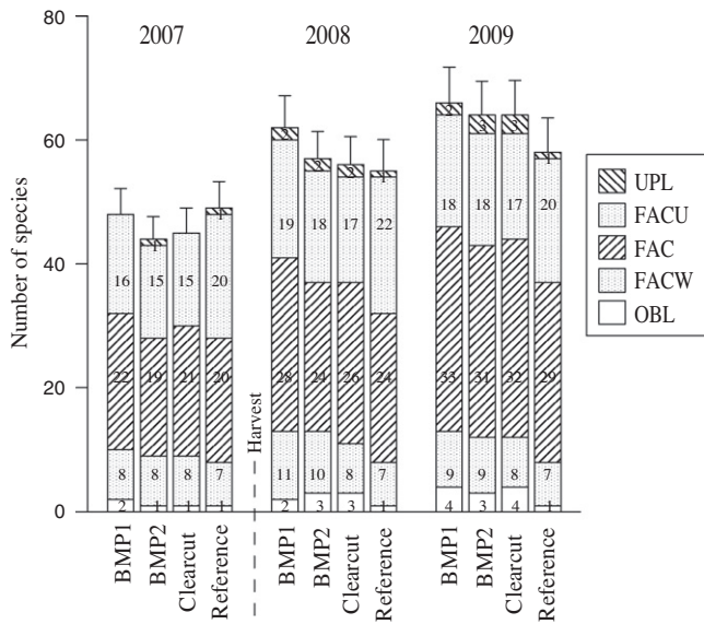
Fig. 3. Proportion of species by wetland indicator classes within treatments by year in small headwater streams of Webster County, Mississippi.
