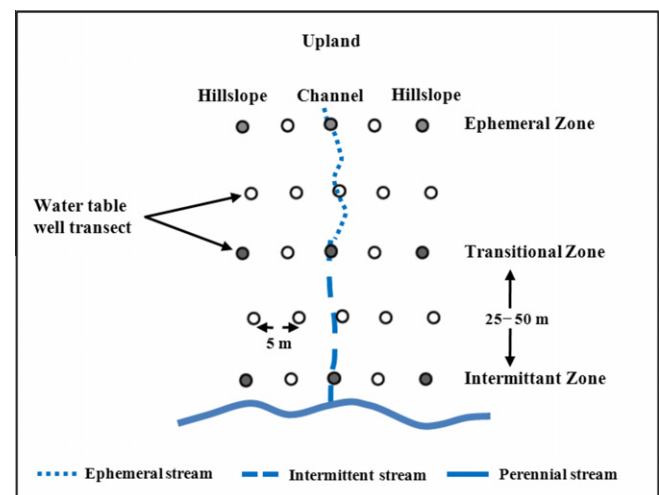
Fig. 1. Schematic of field sampling design in the study watersheds of Webster County, Mississippi. Water table wells served as the center for vegetation sampling strata. Vegetation plots used to calculate prevalence index (PI) are indicated by grey circles located at the 1st, 3rd, or 5th wells of the 1st, 3rd, or 5th transects.
